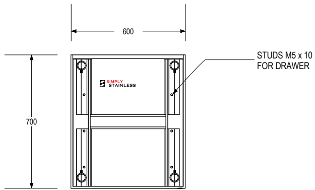
BOTTOM-PLAN VIEW (TOP ONLY)
